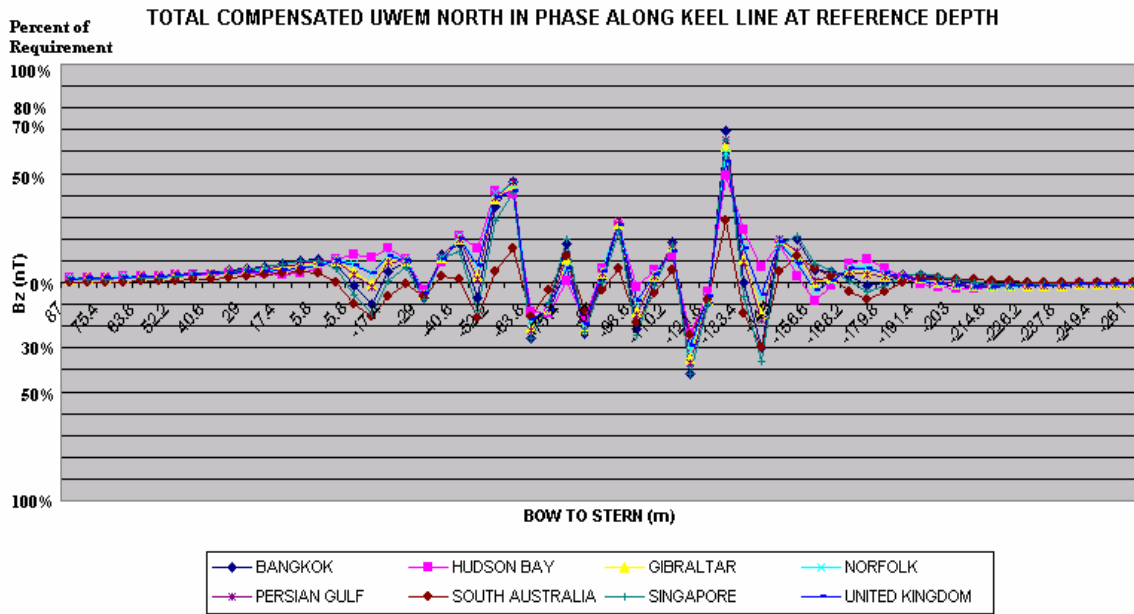
Figure 8 Total Compensated In-Phase UM Signature Along Keel Line, For Various Worldwide Locations, North Heading
