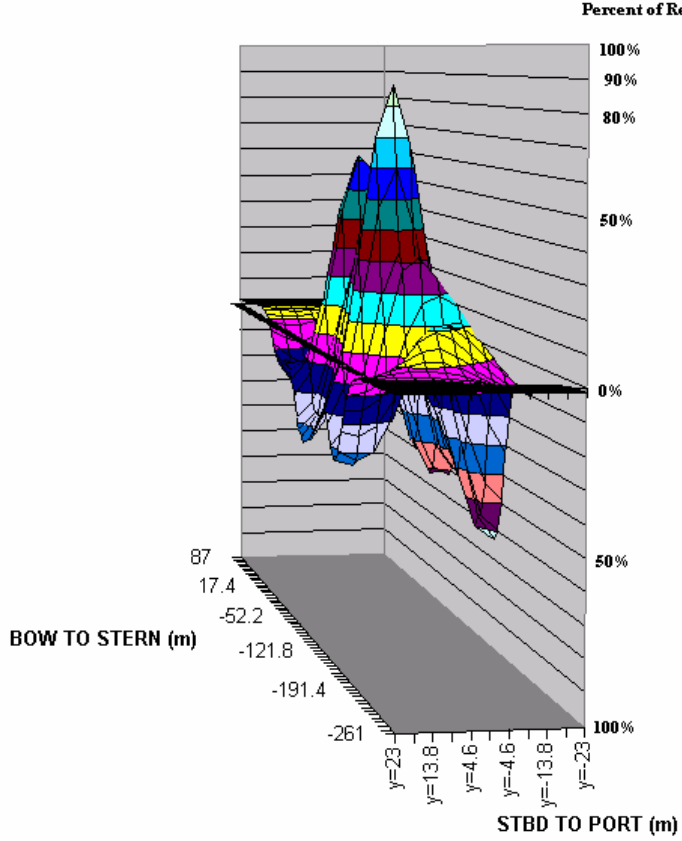
Figure 10 Total Compensated In-Phase UM Signature At Gibraltar, West Heading, At Reference Depth
