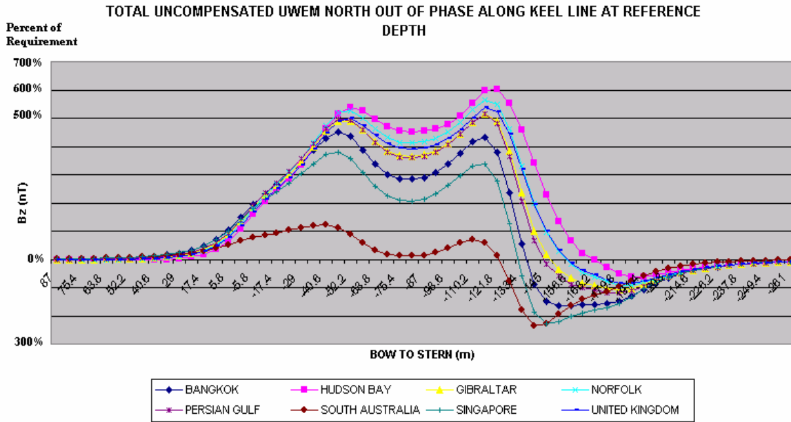
Figure 7 Total Uncompensated Out-Of-Phase UM Signature Along Keel Line, For Various Worldwide Locations, North Heading
