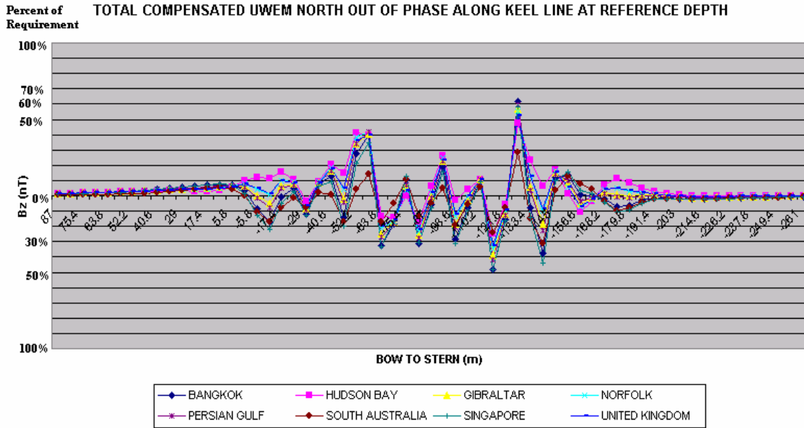
Figure 9 Total Compensated Out-Of-Phase UM Signature Along Keel Line, For Various Worldwide Locations, North Heading
