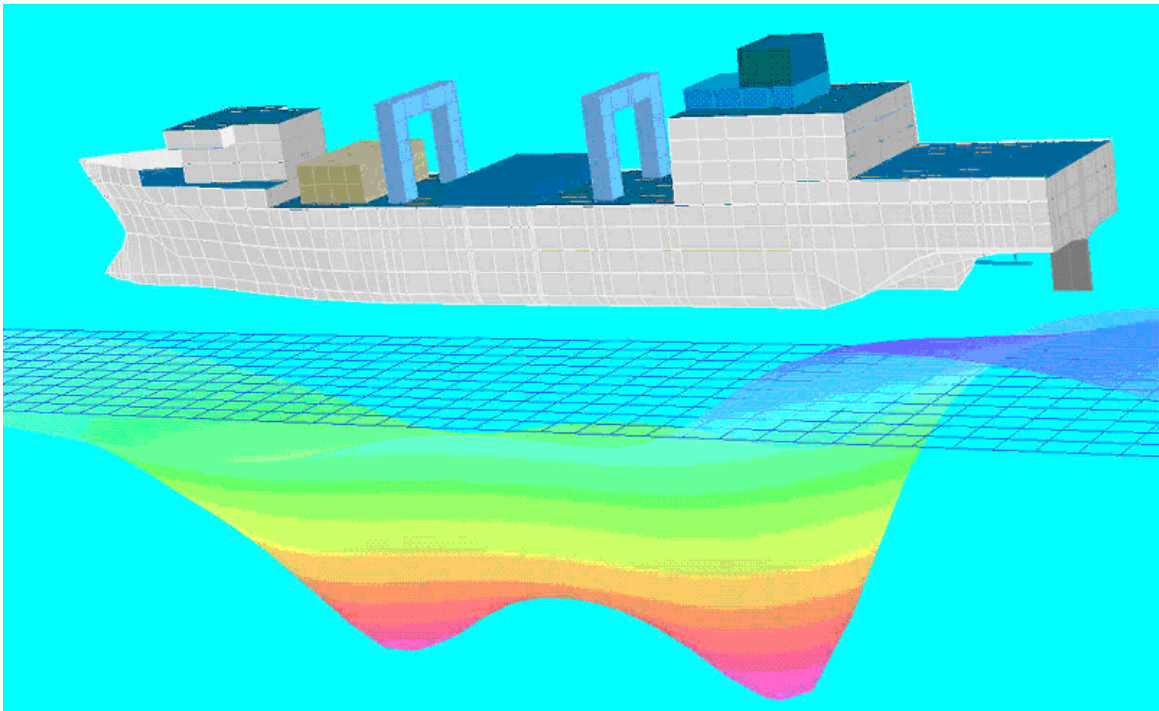
Figure 2 FEM Model Of The Fleet Oiler With The Uncompensated Magnetic Signature At Reference Depth Shown As A 3D Map
