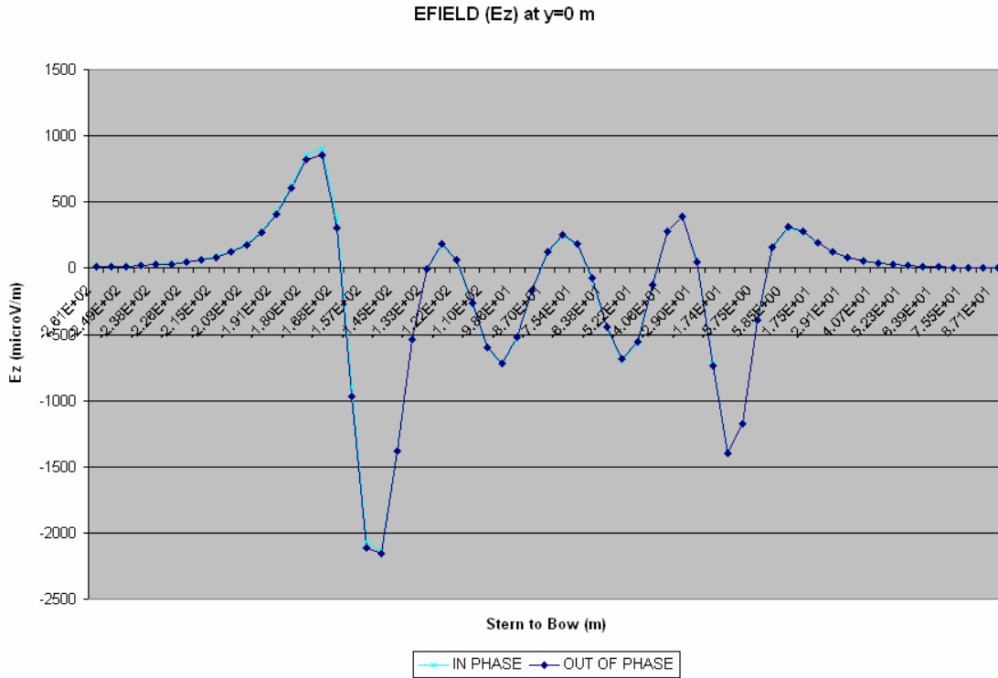
Figure 12 Total Compensated In And Out-Of-Phase UE Signature, All Headings, At Reference Depth
