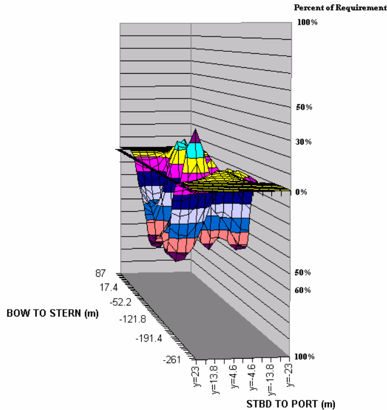
Figure 11 Total Compensated Out-Of-Phase UM Signature At Gibraltar, West Heading, At Reference Depth
