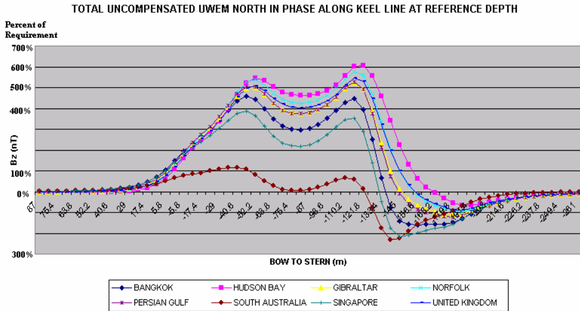
Figure 6 Total Uncompensated In-Phase UM Signature Along Keel Line, For Various Worldwide Locations, North Heading
