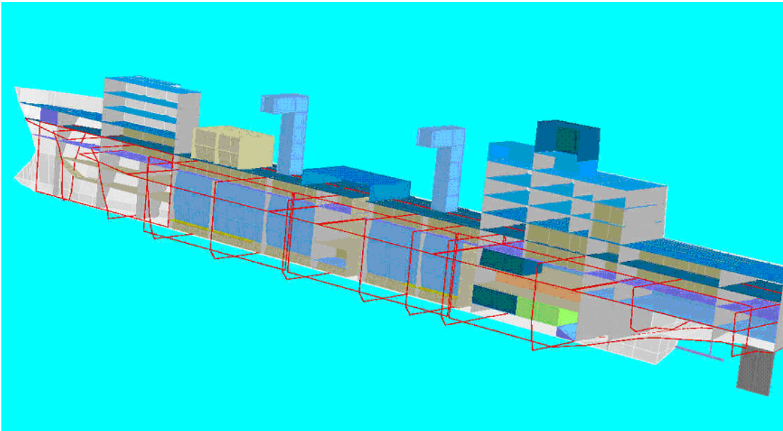
Figure 3 FEM Half-Model Of The Fleet Oiler With MAL DG Coil Runs Shown In Red
