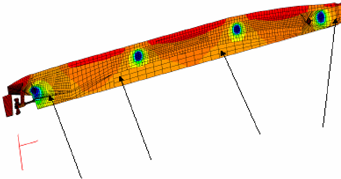
Figure 5 BEM Half-Model Of Fleet Oiler With Hull Potential Distribution (17% Damage), Anodes, And Reference Cell Locations (Arrows) Shown
