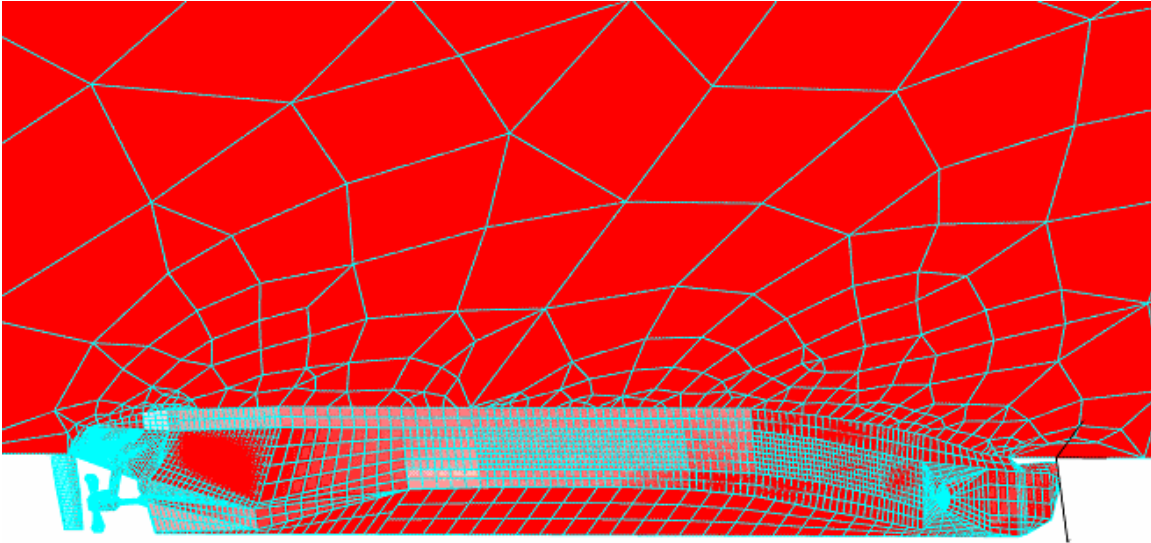
Figure 4 BEM Half-Model Of Fleet Oiler With Sea Surface And Propellers Modeled
